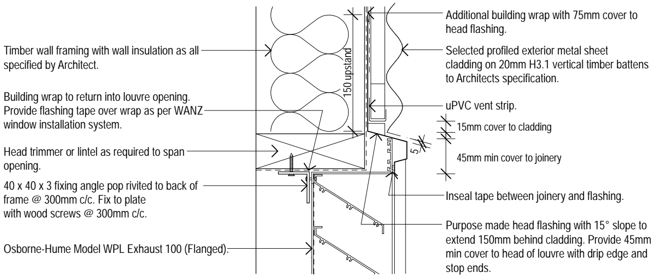
Model Exhaust 100 Louvre (Flanged Frame) Typical Horizontal Corrugate/Louvre Head Detail 01 Osborne-Hume Grilles & Louvres Ltd Scale 1:5
