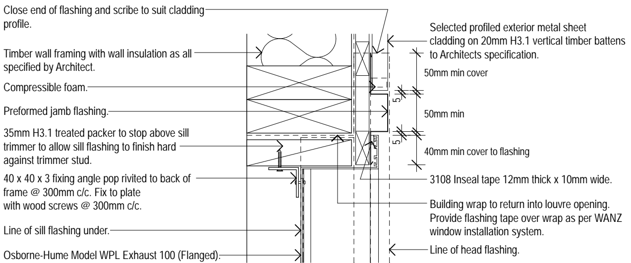
Model Exhaust 100 Louvre (Flanged Frame) Typical Horizontal Corrugate/Louvre Jamb Detail 02 Osborne-Hume Grilles & Louvres Ltd Scale 1:5
