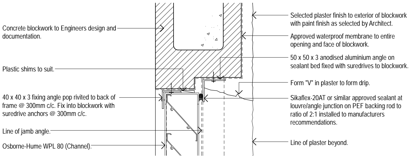
Model WPL 80 (Channel Frame) Typical Blockwall/Louvre Head Detail 01 Osborne-Hume Grilles & Louvres Ltd Scale 1:5
