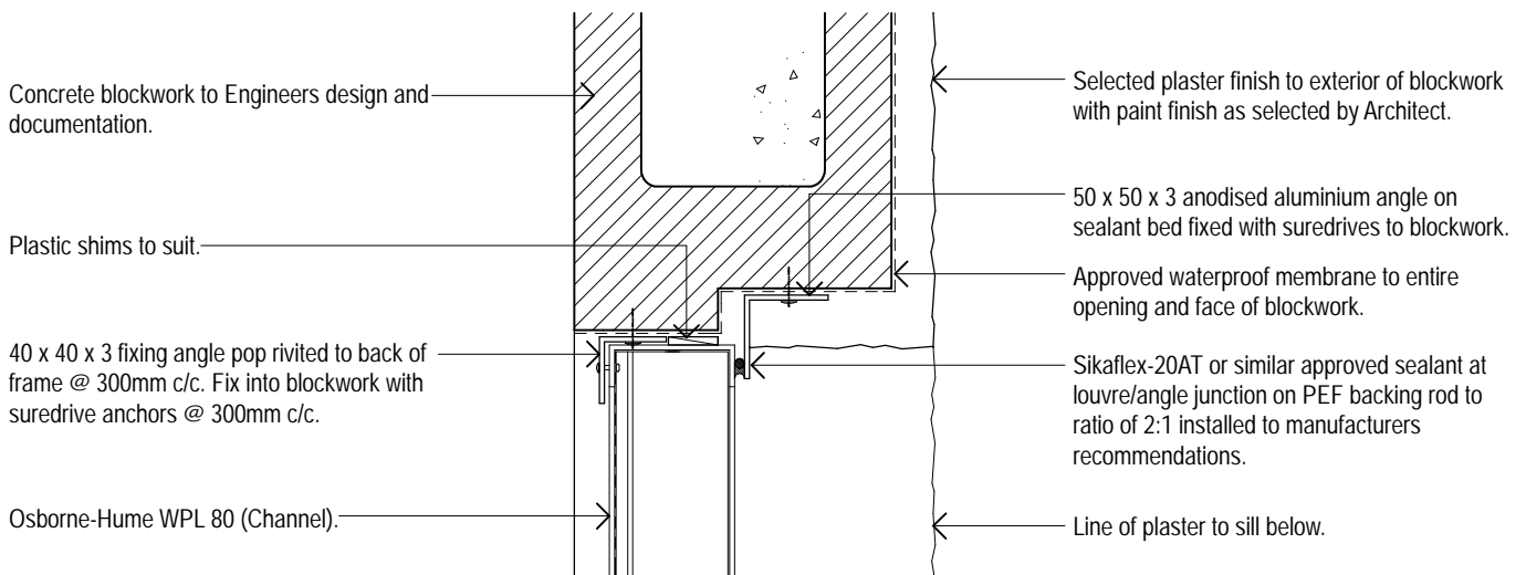
Model WPL 80 (Channel Frame) Typical Blockwall/Louvre Head Detail 01 Osborne-Hume Grilles & Louvres Ltd Scale 1:5
