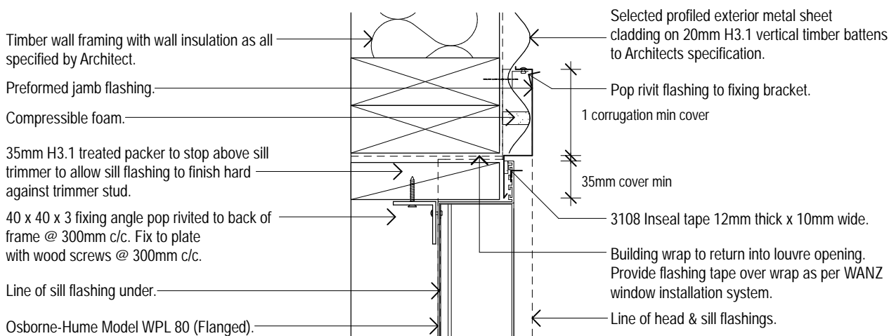
Model WPL 80 (Flanged Frame) Typical Vertical Corrugate/Louvre Jamb Detail 02 Osborne-Hume Grilles & Louvres Ltd Scale 1:5
