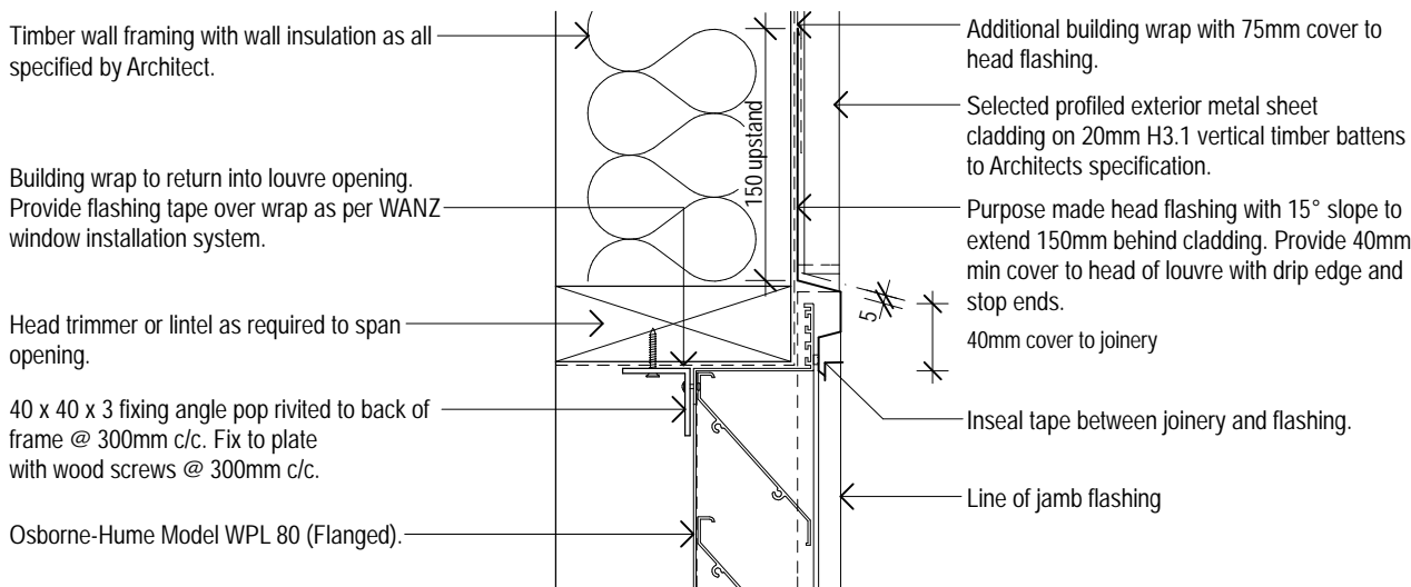
Model WPL 80 (Flanged Frame) Typical Vertical Corrugate/Louvre Head Detail 01 Osborne-Hume Grilles & Louvres Ltd Scale 1:5
