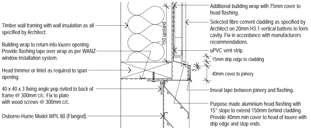
Model WPL 80 (Flanged Frame) Typical Fibre Cement/Louvre Head Detail 01 Osborne-Hume Grilles & Louvres Ltd Scale 1:5
