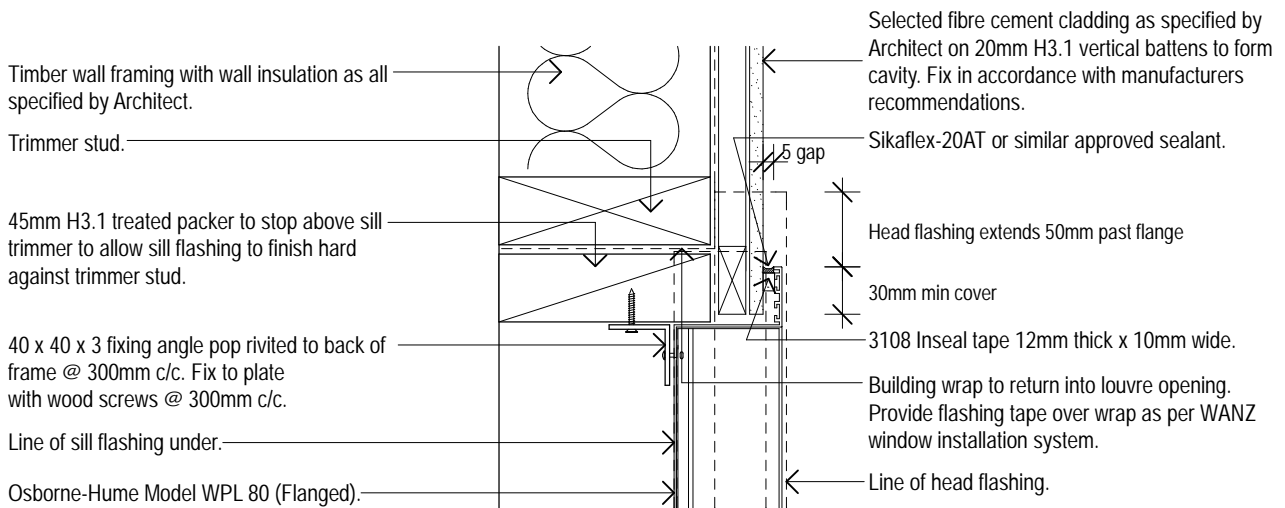
Model WPL 80 (Flanged Frame) Typical Fibre Cement/Louvre Jamb Detail 02 Osborne-Hume Grilles & Louvres Ltd Scale 1:5
