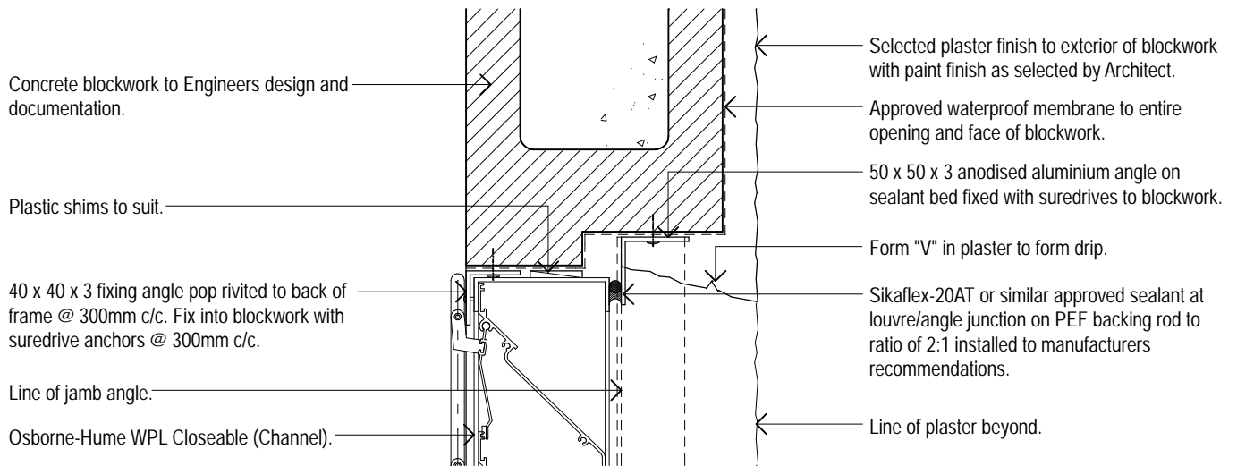
Model WPL Closeable (Channel Frame) Typical Blockwall/Louvre Head Detail 01 Osborne-Hume Grilles & Louvres Ltd Scale 1:5
