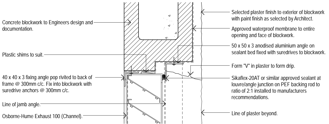
Model Exhaust 100 Louvre (Channel Frame) Typical Blockwall/Louvre Head Detail 01 Osborne-Hume Grilles & Louvres Ltd Scale 1:5
