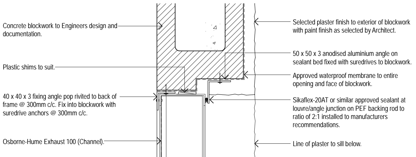
Model Exhaust 100 Louvre (Channel Frame) Typical Blockwall/Louvre Jamb Detail 02 Osborne-Hume Grilles & Louvres Ltd Scale 1:5
