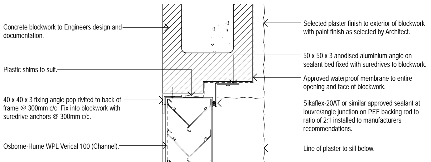
Model WPL Vertical 100 (Channel Frame) Typical Blockwall/Louvre Head Detail 01 Osborne-Hume Grilles & Louvres Ltd Scale 1:5
