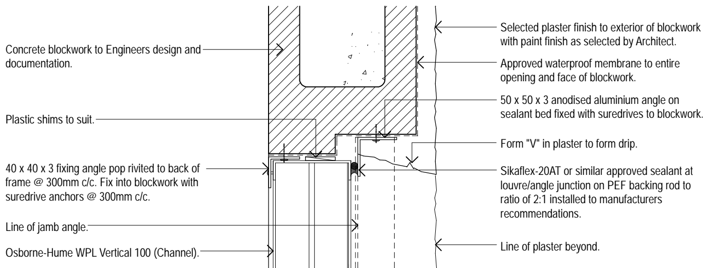
Model WPL Vertical 100 (Channel Frame) Typical Blockwall/Louvre Head Detail 01 Osborne-Hume Grilles & Louvres Ltd Scale 1:5
